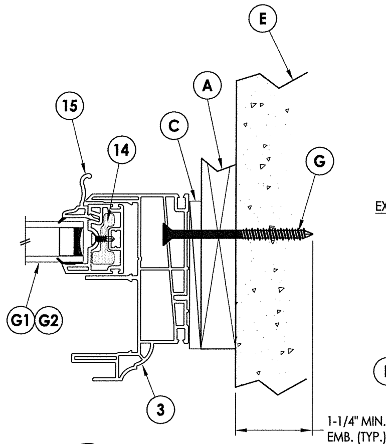
2/2 HORIZONTAL CROSS SECTION 1X Buck Masonry Construction
