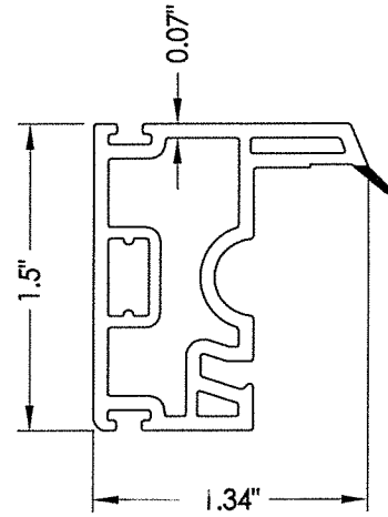
5 MEETING STILE
