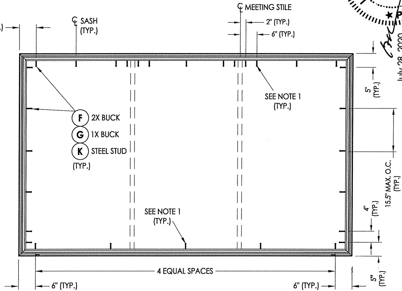
FRAME ANCHORING
